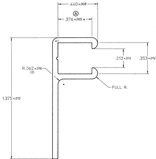
Perpendicular Strip Holder
