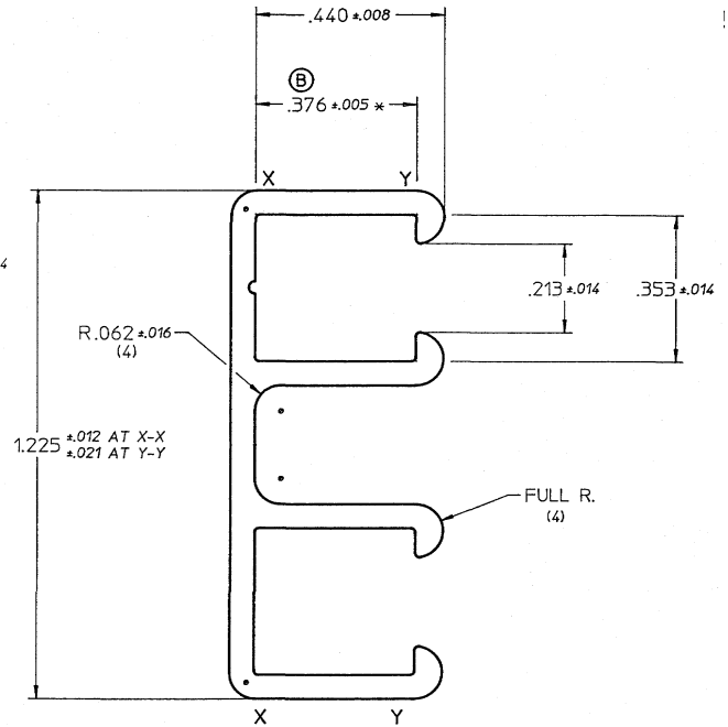
Dual Strip Holder
