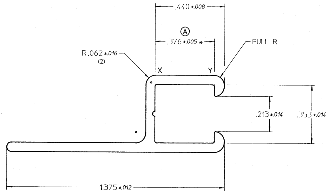
Inline Strip Holder
