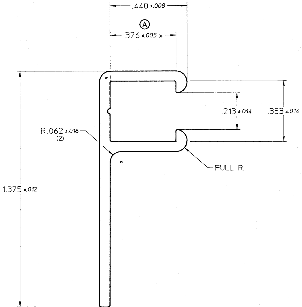
Diagram #1 - Single "b" Strip Holder
