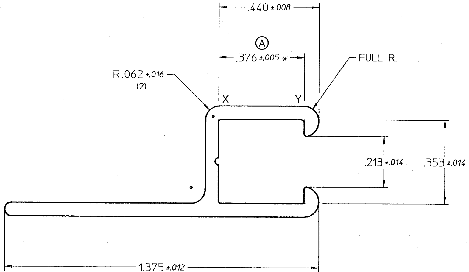
Diagram #1 - Single "h" Strip Holder
