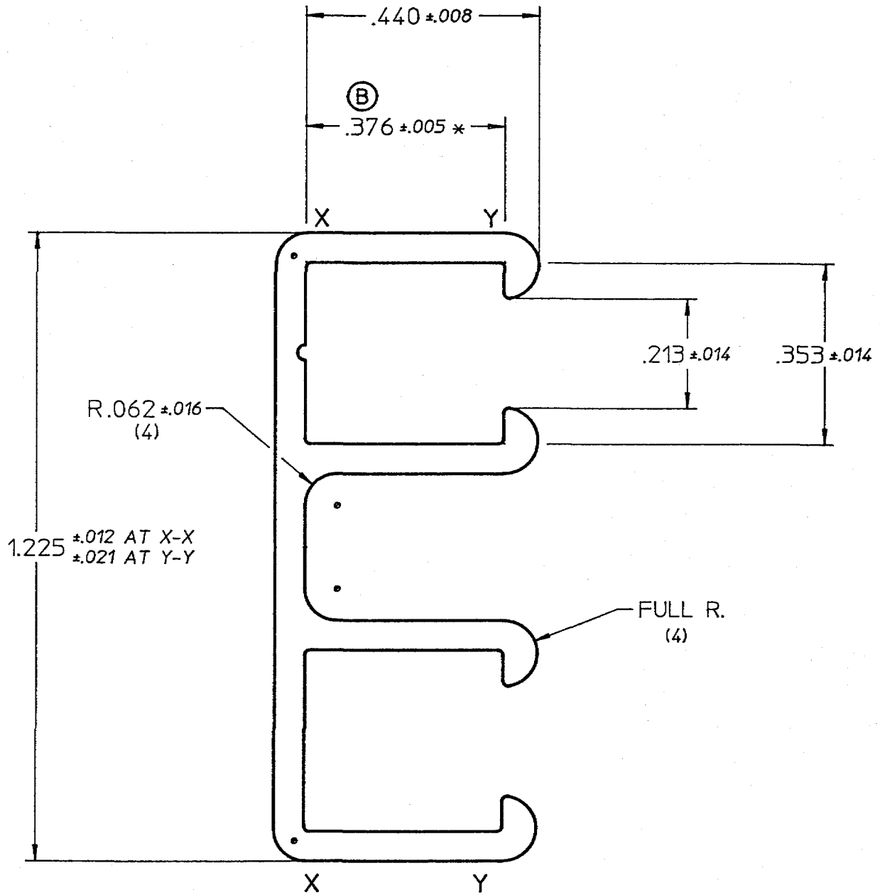
Diagram #1 - Dual Strip Holder
